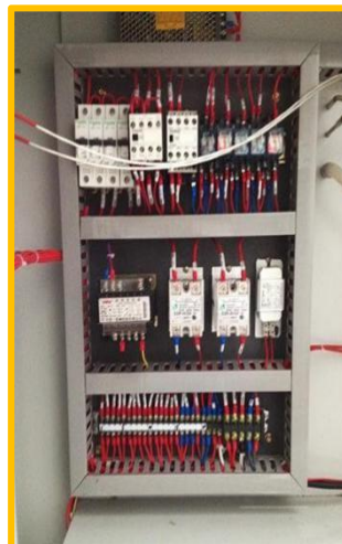
Circuit system
