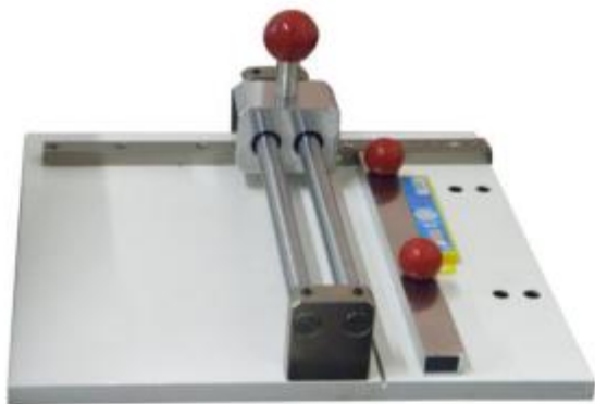
SAMPLER DEVICE OF Edge Compression Test (ECT) / Peel Adhesive Test (PAT)
